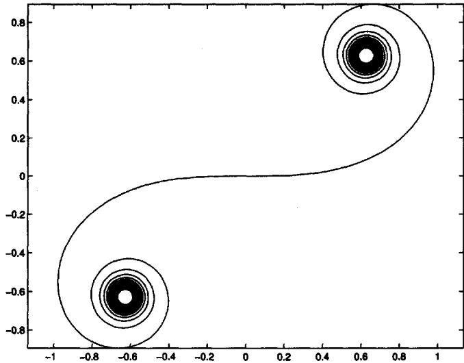
Figure 12.2. Fresnel spiral.
