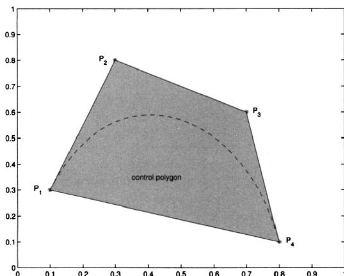
Figure 8.9. Bezier curve and control polygon.
