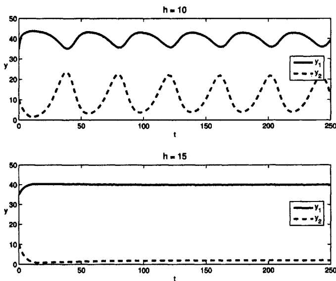
Figure 12.17. Predator-prey model with delay and harvesting.
