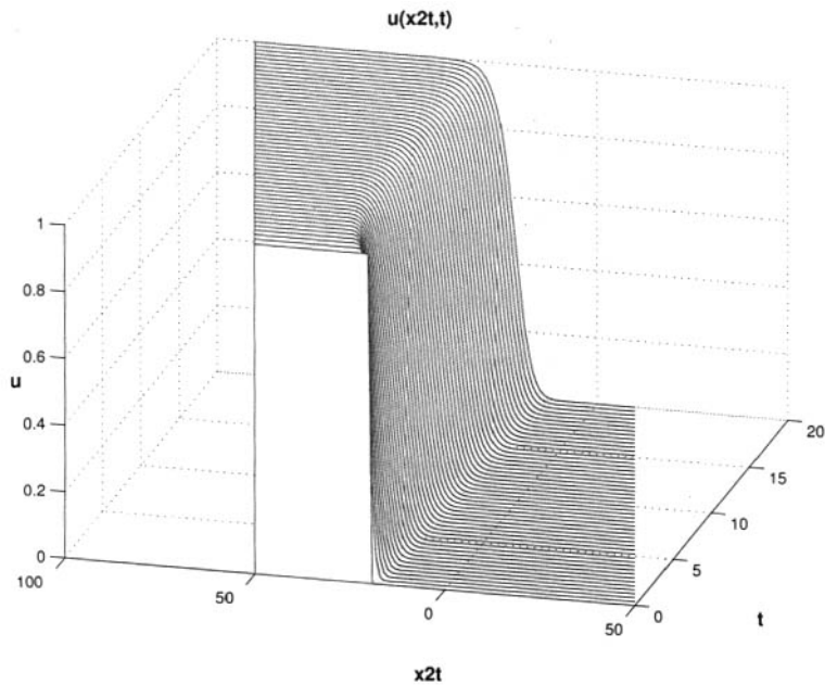
Figure 22.12. Solution of Fisher's equation for initial conditions (22.10) in moving coordinate system, from fisher.
