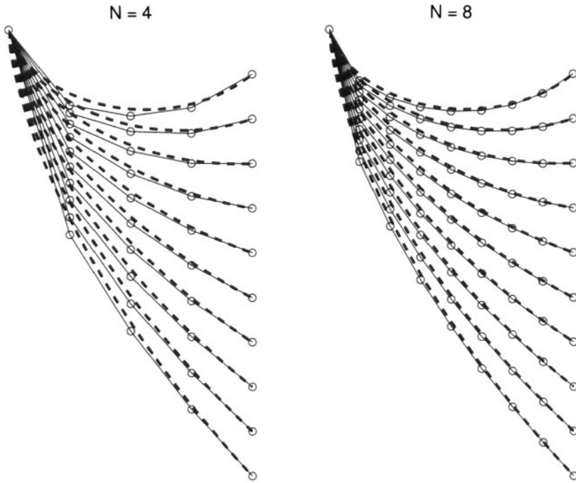
Figure 22.1. Output from brach.
