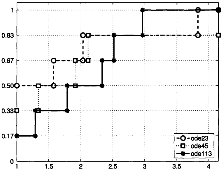
Figure 22.3. Performance profile produced by ode_pp.
