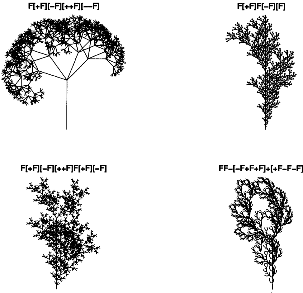
Figure 22.6. Members of the genus Matlabius Floribundum produced by 1sys.
