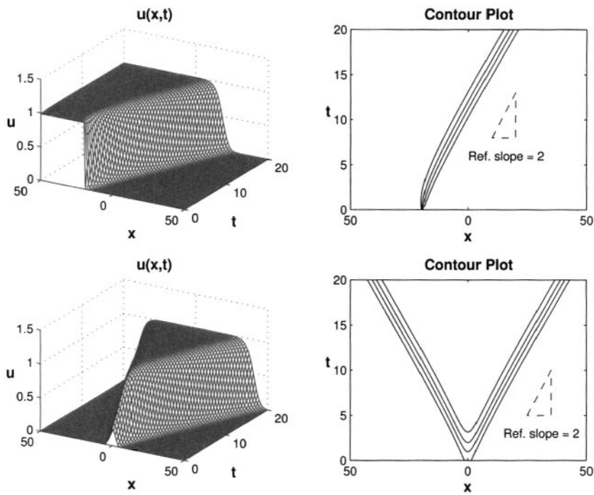
Figure 22.11. Traveling wave solutions for Fisher's equation, from fisher.
